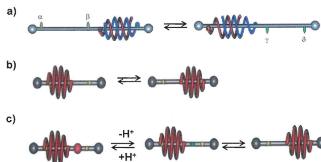
Figure 3. a) Foldaxane shuttling on a rod-shaped guest molecule that has two nondegenerate binding stations. b) Single helical foldaxane shuttling on a rod-shaped guest molecule that has two degenerate binding stations. c) Helix shuttling in response to pH.
